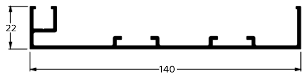
MARCO LATERAL PERSIANA
