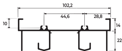
LG-044 1,247 KG/M
