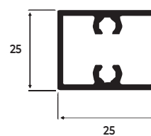
TRAVESSA / MARCO
