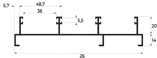
LG-064 1,358 KG/M
