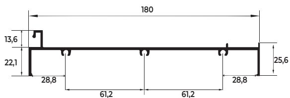
LG-041 1,370 KG/M
