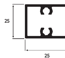
TRAVESSA / MARCO
